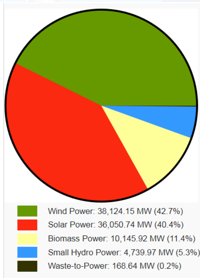
Fig: Installed grid-interactive renewable power capacity in India as of 30 September 2020 (excluding large hydro)
